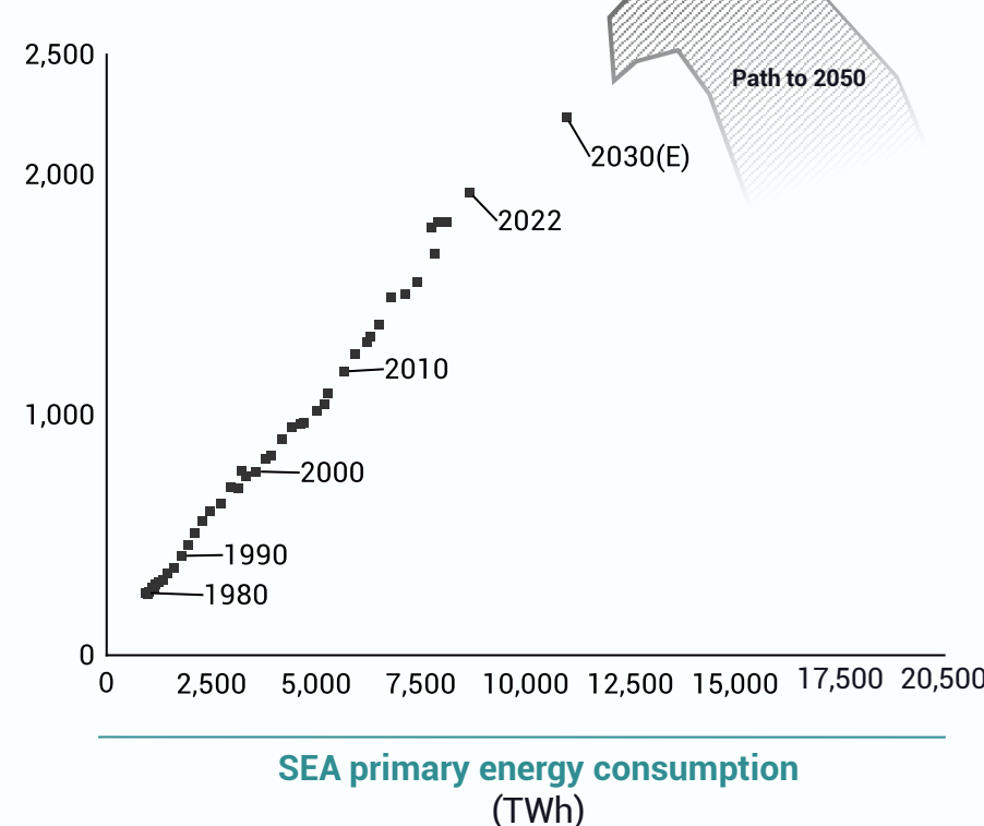
SEA CO 2 emissions 2 (Mt)
